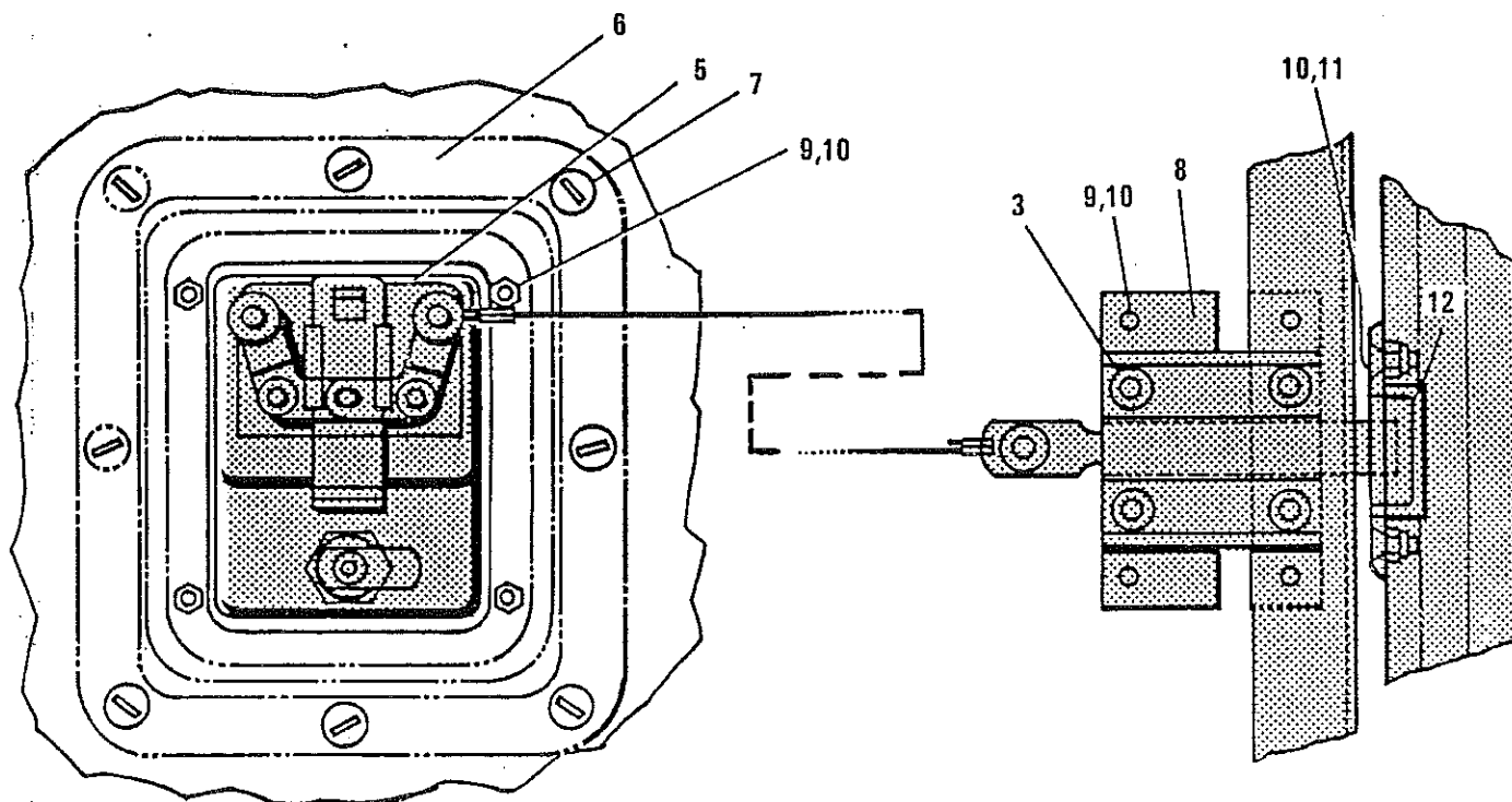
REAR LATCHING MECHANISM, AS SEEN FROM INSIDE TRUCK
