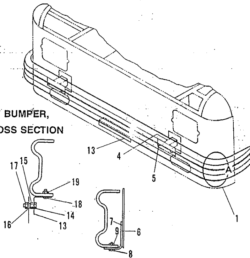
CROSS SECTION, AREA A
