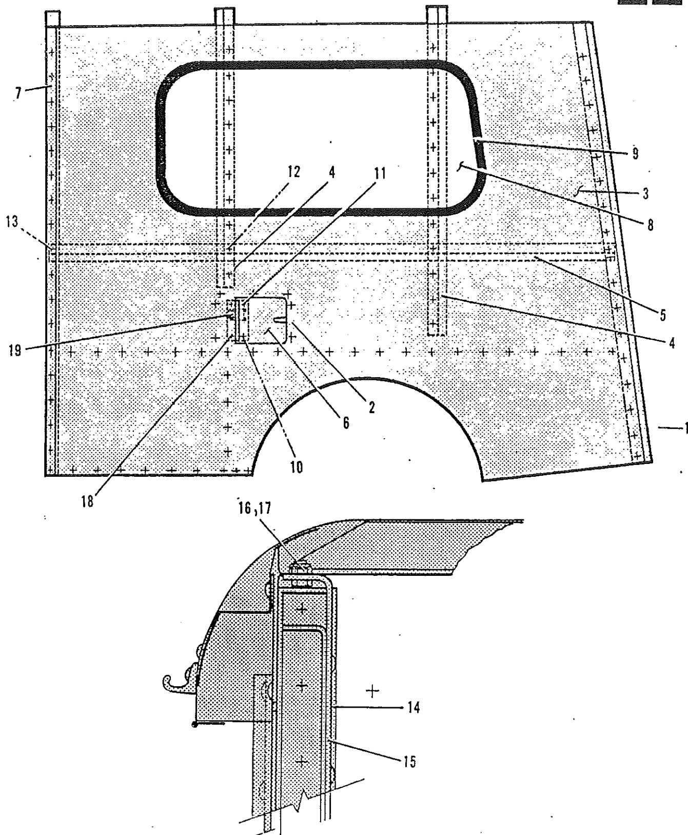
CROSS SECTION, L.H. DOOR POST, LOOKING FORWARD
